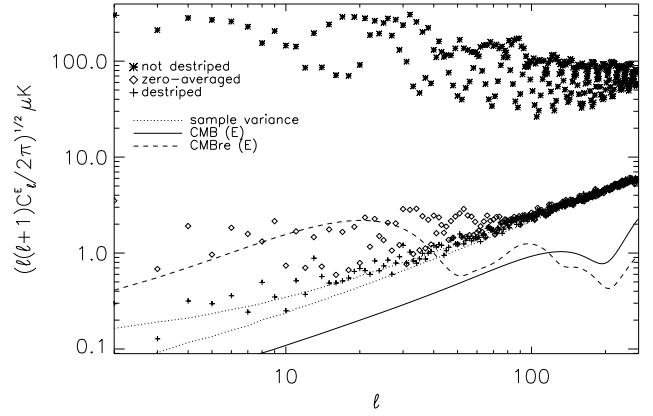
Fig. 15. Efficiency of destriping for the E field for f_{\text{knee}}/f_{\text{spin}} = 1 . The zero-averaged spectrum is not as bad as for T but the residual striping we can see in Fig. 12 leads to some excess of power for low values of \ell (up to \ell \sim 100 ). We do not see such effect in the destriped spectrum (and maps). The spectra for the B fields are very similar. The solid line represents a standard CDM E spectrum and the dashed line represents a CDM E spectrum with reionization.
