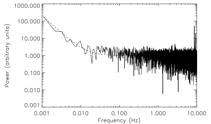
Fig. 1. The power spectrum of the K34 bolometer from Caltech, the same type of bolometer planned to be used on the PLANCK mission. The measurement was performed at the SYMBOL test bench at I.A.S., Orsay (supplied by Michel Piat). The knee frequency of this spectrum is \sim 0.014 Hz and the planned spin frequency for PLANCK is 0.016 Hz. We can model the spectrum as the function S(f) = 1 + \left(\frac{1.43 \times 10^{-2}}{f}\right)^2 (dashed line).
