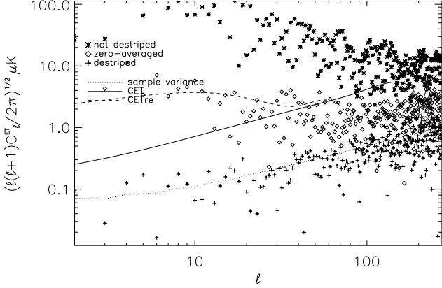
Fig. 17. Same as Fig. 15 for the ET -correlation for f_{\text{knee}}/f_{\text{spin}} = 1 .
