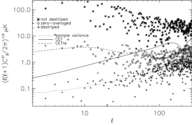
Fig. 18. Same as Fig. 17 but for f_{\text{knee}}/f_{\text{spin}} = 5 .
